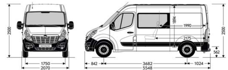
Opel Movano Crew Van FWD L2H2
