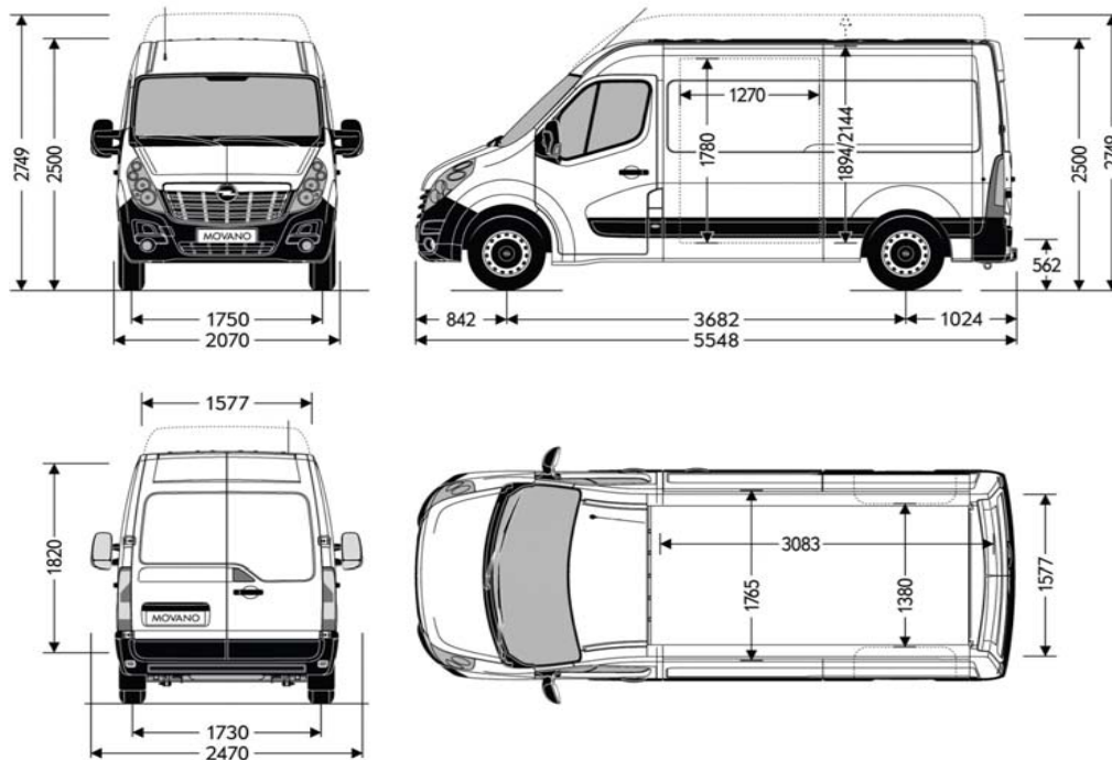
Opel Movano Van FWD L2H2-H3
