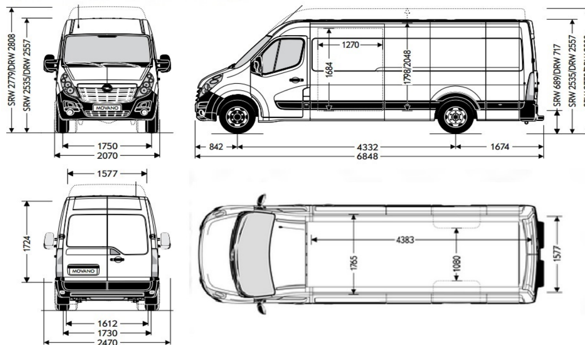
Opel Movano Van RWD L4H2-H3
