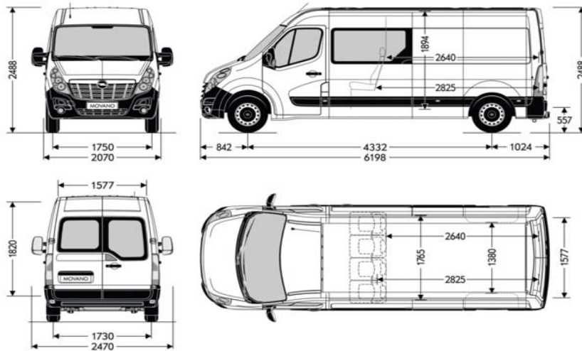
Opel Movano Crew Van FWD L3H2
